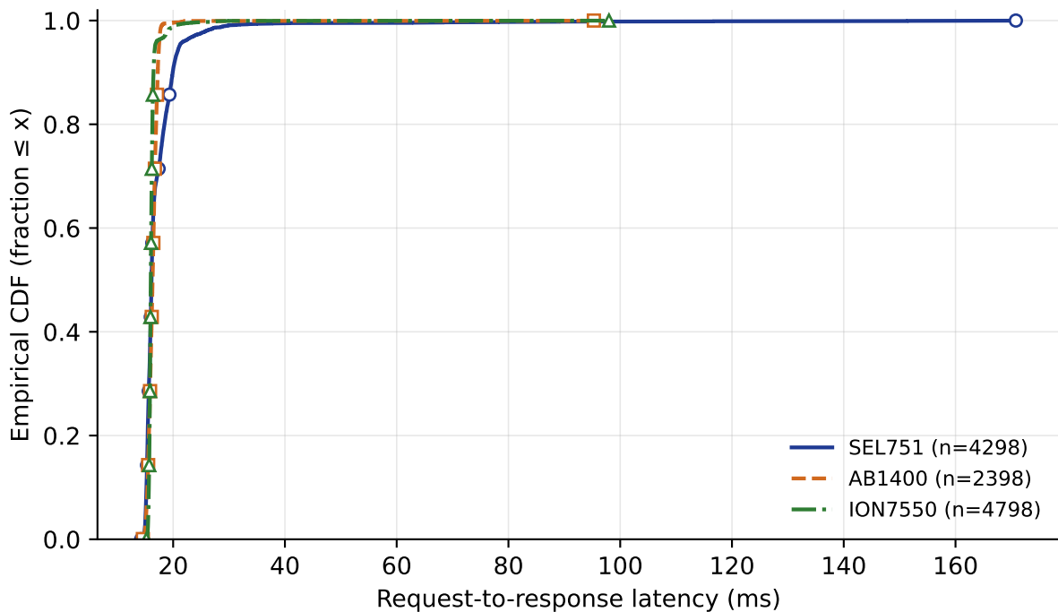
Request-to-response latency CDF by device (n=11494; SEL751=4298, AB1400=2398, ION7550=4798)
