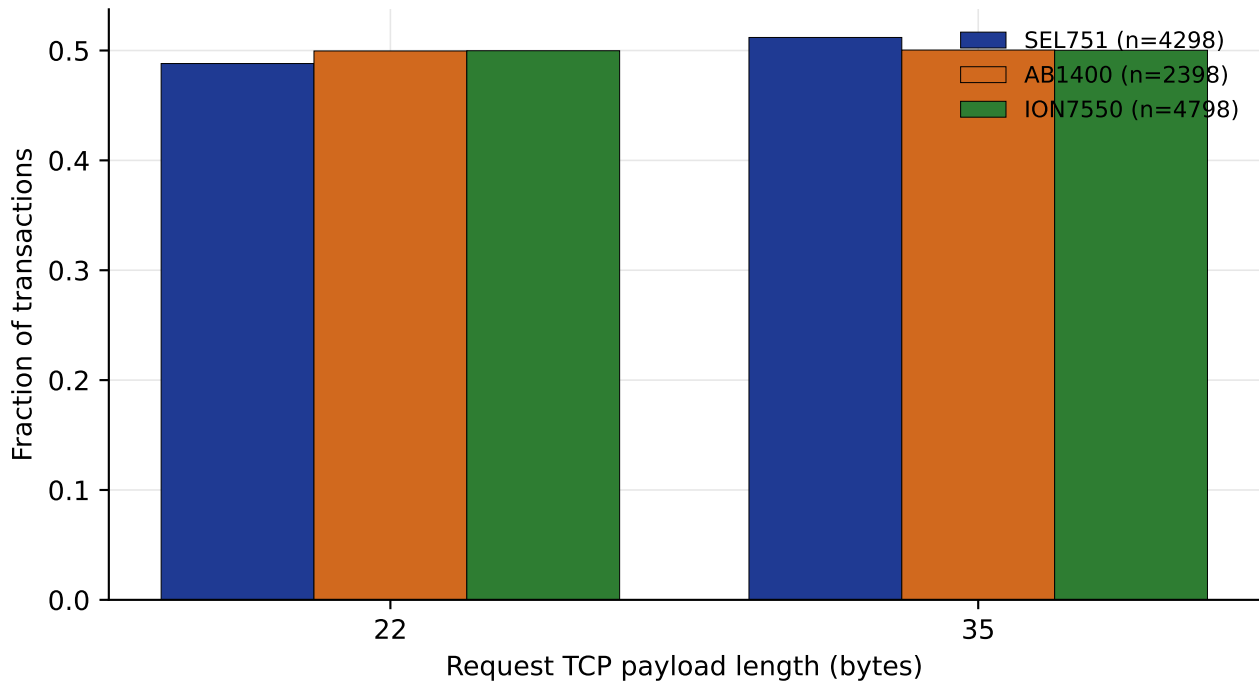
Request-size distribution by device (n=11494)
