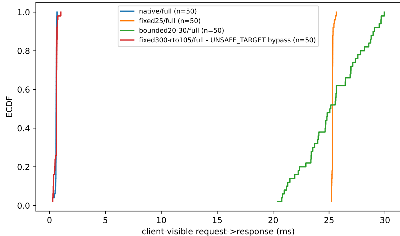
Phase 02: client-visible time ECDF by config (2407 B READ, full delivery)
