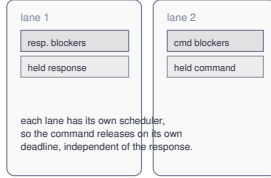
Fig. 6. Why two scheduling lanes are needed. (a) On one shared strict-priority schedule, the response's blocker packets starve the held control command below them, so its release drifts to the response's release time. (b) Two independent lanes each carry their own blockers and held packet, so the command releases on its own deadline. Both lanes are internal to the same switch and program.
