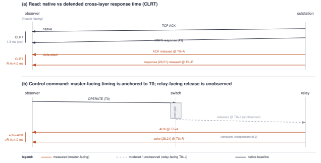
Fig. 7. Native versus defended timing, and the control-command timeline. The defended acknowledgment and response are placed at T_0 + A and T_0 + R ; the internal release at T_0 + J is on the relay-facing link and is not captured (dashed), so it is verified by the model rather than measured.
