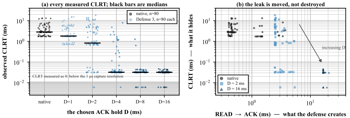
Figure 12: (a) Every measured CLRT, one point per transaction, 80 per arm, on a logarithmic axis; black bars are medians and points are jittered horizontally only. The native cloud spans 1.7–13.2 ms; by D = 16 ms it has compressed onto an external floor of about 32 \mu s (median 0.0319 ms, sd 0.0120, max 0.0470 — a tight distribution, not a constant). Points in the grey band were measured as exactly zero, i.e. below the 1 \mu s resolution of the capture. (b) The same data plotted as the two observables against each other. The native cloud sits at the left, spread vertically — the vertical spread is the fingerprint. As D grows the cloud moves right and flattens: the spread leaves the CLRT axis and appears on the READ \rightarrow ACK axis. Nothing is destroyed; it is moved. Source: figures/src/fig7_scatter.py .
