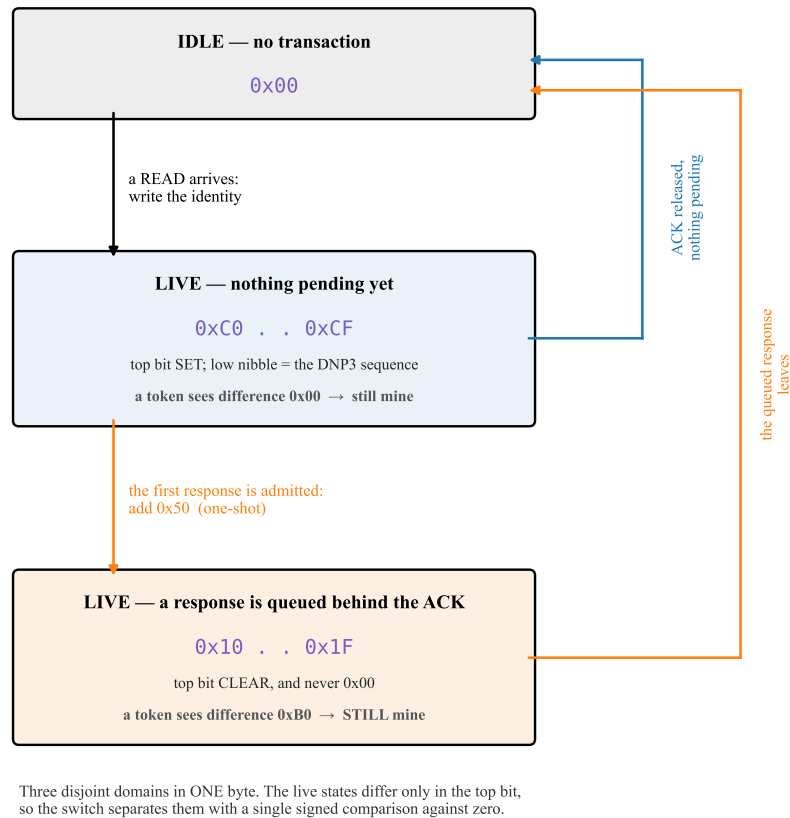
Figure 10: The transaction state machine: three disjoint domains inside one byte. The two live states differ only in the top bit, so the switch separates them with a single signed comparison against zero (§8). The white lines inside the live boxes are what a circulating blocker token computes — the identity it carries minus the value it finds. Because the marking transition adds a constant rather than overwriting, that difference is 0x00 before marking and 0xB0 after, so one extra table entry covers all sixteen identities and the reservoir survives the state change. Source: figures/src/fig5_statemachine.py.
