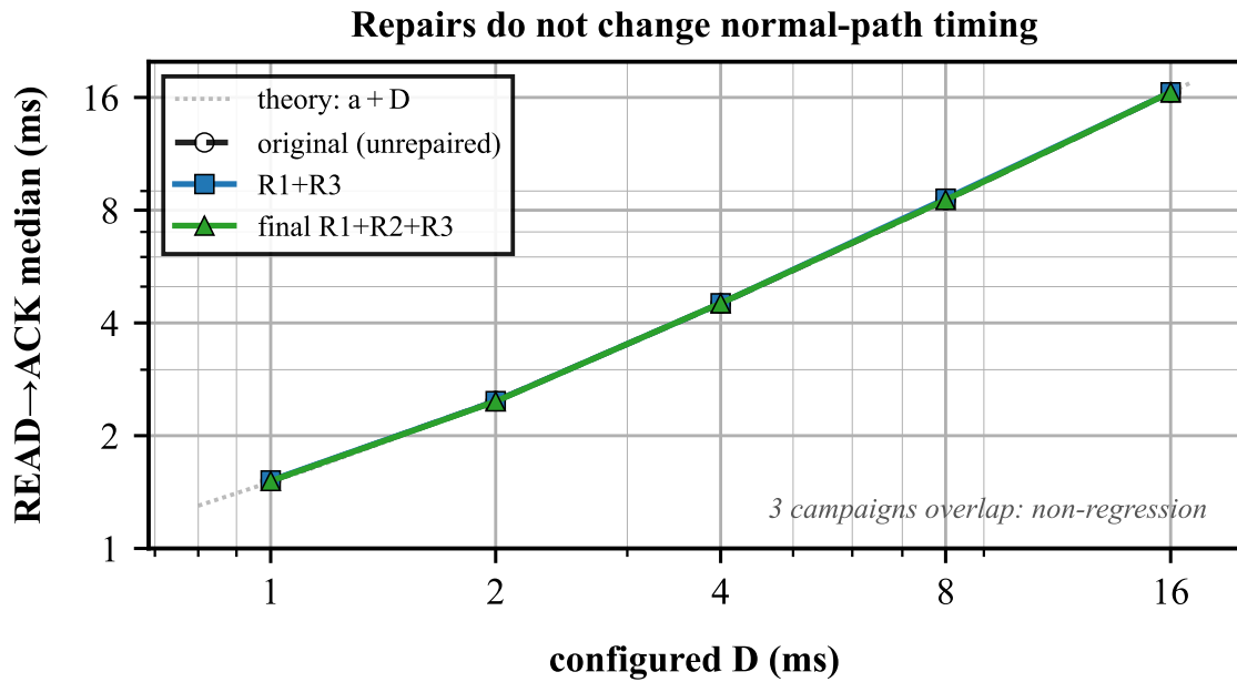
Figure 11: The repairs changed correctness without moving the normal-path timing. READ→ACK median vs D for all three physical campaigns (original unrepaired, R1+R3, and the final R1+R2+R3) lie almost on top of each other and on the theoretical a + D : at D = 16 ms the three medians are 16.509/16.510/16.512 ms. This is the non-regression result an eavesdropper’s wire view confirms.
