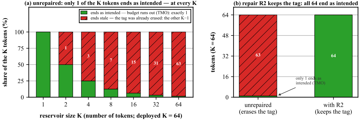
Figure 9: The fail-open reconciliation. (a) On the unrepaired build the budget-zero terminations are 1 (budget) and K - 1 (stale) at every reservoir size, including K = 1 — one native token clears reg_tag and the rest read foreign, so the defect is not an emergent effect of size. (b) R2 turns the same event into K budget terminations and 0 stale, and preserves reg_tag . Source: figures/src/fig9_ksweep.py.
