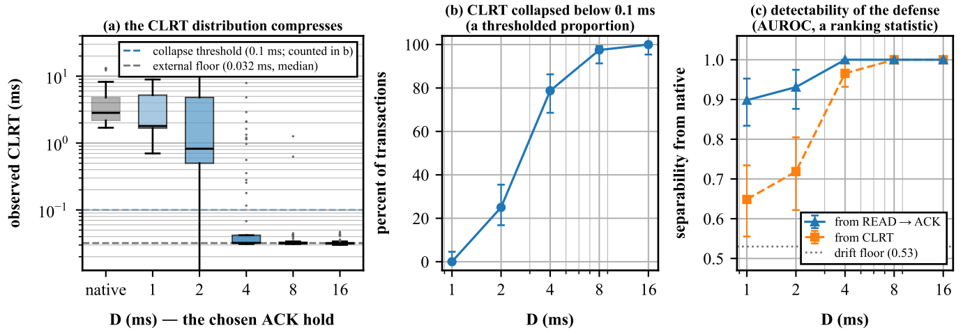
Figure 13: The central result: 480 transactions against the real relay, 400 of them defended. (a) The observed CLRT distribution per arm on a log scale. The distribution compresses onto an external floor of about 0.032 ms — the gray dashed line — as D grows past the relay’s own response time; that floor is the master-capture ACK→RESPONSE gap, not the switch’s 26 ns internal release tail, and it is a tight distribution rather than a constant. (b) The percentage of transactions whose CLRT falls below 0.1 ms — a thresholded sample proportion. (c) How well an adversary separates defended from undefended traffic using each feature — a ranking statistic (AUROC). Error bars are 95 % confidence intervals: a Wilson score interval for the proportion in (b), a bootstrap percentile interval for the AUROC in (c). (b) and (c) are different kinds of quantity and must not be compared arithmetically, so they are separate panels. The dotted line in (c) is the native-versus-native drift floor, 0.53, which is what “no information” looks like in this session. Collapse and detectability rise together, and detection is already near-perfect where the collapse is only partial. Source: figures/src/fig1_dsweep.py.
