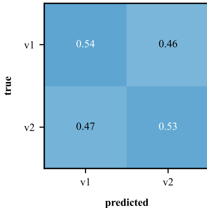
Defended (random J) RF acc=0.53
