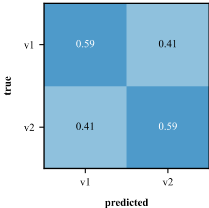
Native (no defense) RF acc=0.59
