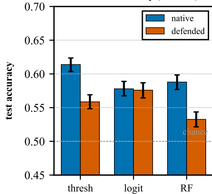
Two-class accuracy (95% CI)
