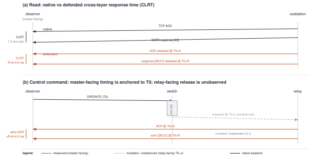
Fig. 4. Native versus defended timing, and the control-command timeline. The defended acknowledgment and response are placed at T_0 + A and T_0 + R ; the internal release at T_0 + J is on the relay-facing link and is not captured (dashed), so it is verified by the model rather than measured.
