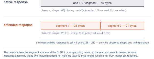
Fig. 2. Native versus defended, as observed. The native response is one 49-byte segment with variable timing; the defended response is the same 49 bytes as a fixed [28, 21] two-segment shape with a fixed CLRT. The total length is unchanged.
