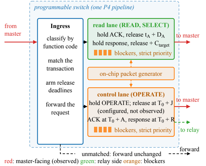
Fig. 4. How one pipeline realizes the schedule. Ingress classifies each DNP3 transaction and arms its release deadlines. The read lane holds the acknowledgment and the response of a READ or SELECT and releases them relative to the outstation's acknowledgment; the control lane holds an OPERATE, releases it toward the relay at a configured delay that we do not observe, and releases the acknowledgment and solicited response relative to the request. The packet generator fills the blocker reservoirs (orange), and a strict-priority scheduler drains them before the held packet, which is what sustains a hold until its deadline expires. Red arrows are master-facing and observed; the green dashed arrow is the configured relay-facing release, which is not. Unmatched traffic is forwarded unchanged.
