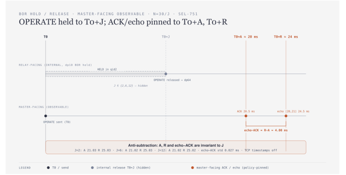
Fig. 4. Master-facing timing of a control command. The ACK and echo are placed at T_0 + A and T_0 + R , anchored to the OPERATE arrival T_0 , so the observable gap R - A is fixed. The internal release at T_0 + J is on the relay-facing link and is not captured (dashed), so it is verified by the implementation model rather than measured.
