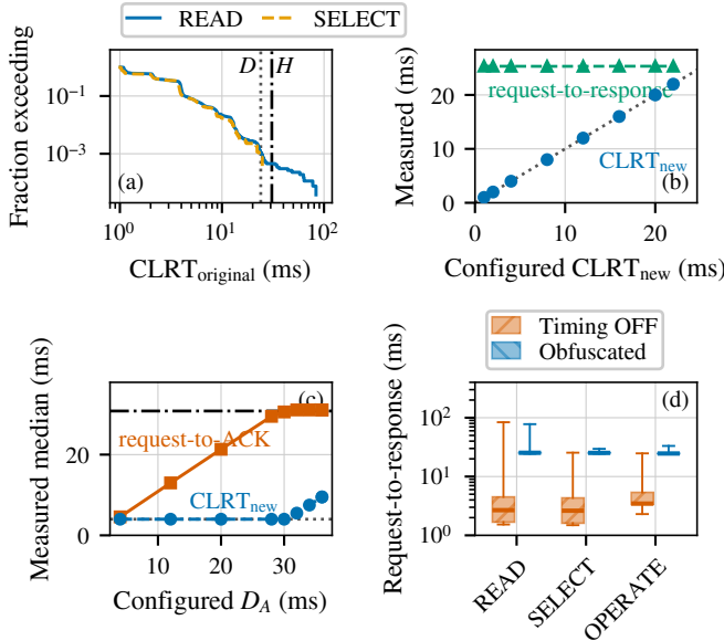
Fig. 9. The release policy is programmable and bounded on both sides. (a) Timing OFF read-lane tail against the budget D and the horizon H . (b) At D = 24 ms the measured CLRT new follows the configured CLRT new while the response latency stays fixed. (c) Raising D_A saturates near H . (d) End-to-end response time per class.
