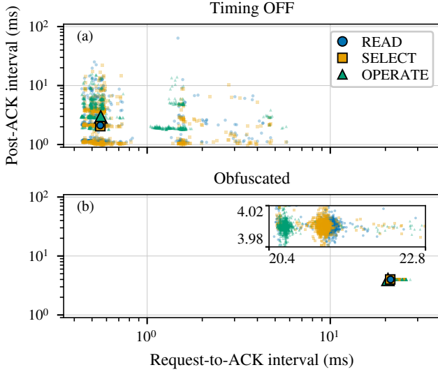
Fig. 10. The two measurable intervals against each other, (a) Timing OFF and (b) Obfuscated. Under the mechanism the vertical interval of all three classes collapses onto the policy value, while OPERATE keeps a horizontal offset because the two lanes are timed from different events. Small marks are a subsample; the outlined marks are class medians over the full dataset.
