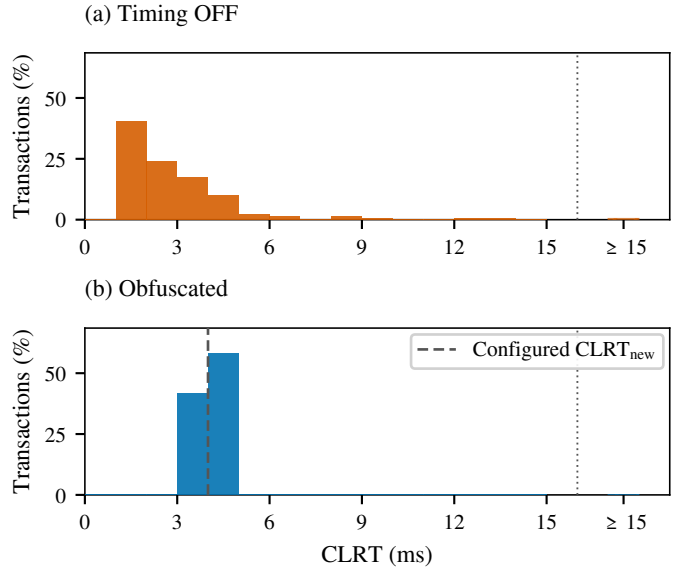
Fig. 5. Measured READ CLRT before and after obfuscation, as the percentage of each arm's own transactions per bin, on common 1 ms bins anchored at 0 ms with a linear ordinate. Finite bins are half-open; the hatched category holds everything at or above 15 ms, 0.409% of (a) and 0.027% of (b). The dashed line in (b) is the configured CLRT new , which falls on a bin edge, so the obfuscated mass divides between the two neighbouring bins; Figure 6 resolves it. In (a) n = 26,400 , mean 2.800 ms, sd 2.609 ms, variance 6.808 ms 2 ; in (b) n = 26,400 , mean 4.012 ms, sd 0.628 ms, variance 0.394 ms 2 .
