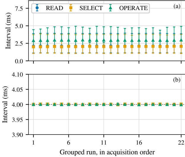
Fig. 8. Per-run medians and interquartile ranges, in acquisition order. Panel (b) uses a magnified ordinate spanning 0.20 ms. The runs are one campaign, not independent replications.
