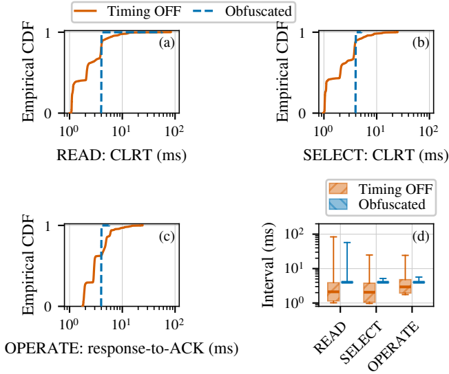
Fig. 7. Measured interval per class. (a) READ and (b) the SELECT phase of SBO report the CLRT; (c) OPERATE reports the master-visible response-to-ACK interval, timed from the request. (d) The same measurements as quartiles. The abscissa is logarithmic and spans the full support.
