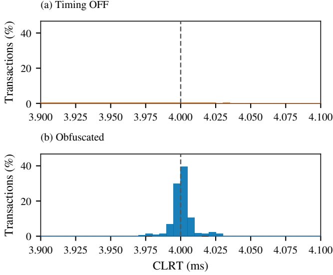
Fig. 6. The released interval, resolved. The same measurements as Figure 5 on 0.005 ms bins within 0.10 ms of the configured CLRT new (dashed). The ordinate is still the percentage of that arm’s entire sample, not of the window, so the bars are directly comparable with the other figures. The window holds 13.58% of (a) and 99.86% of (b).
