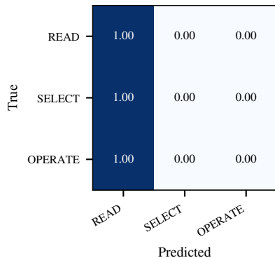
(c) A fixed on Obfuscated, CLRT
