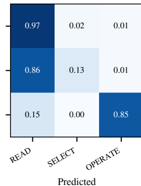
(e) B adaptive on Obfuscated, both
