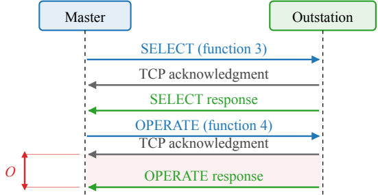
(b) Select-before-operate control
