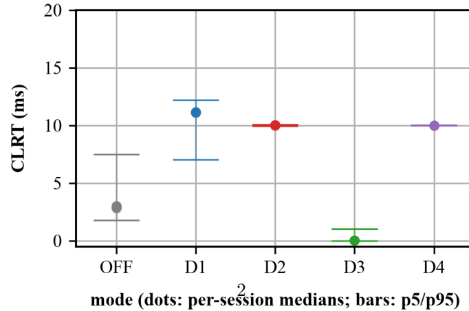
Figure 2: Per-session medians (dots) and pooled p5/p95 (bars) per mode. D2 and D4 are tight at 10 ms and stable across sessions; D1 (event) shifts the distribution but keeps its spread.
