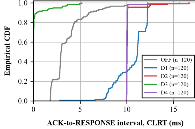
Figure 1: Native (OFF) versus the Defense 4 modes: empirical CDF of the CLRT. OFF is the wide native curve; D2 and D4 are near-vertical steps at 10 ms with a short late tail; D3 collapses to \sim 0 ; D1 shifts to \sim 11 ms. n=120 per mode, Campaign A.
