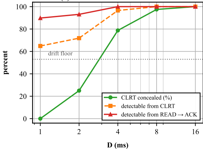
(b) but the defense becomes obvious
