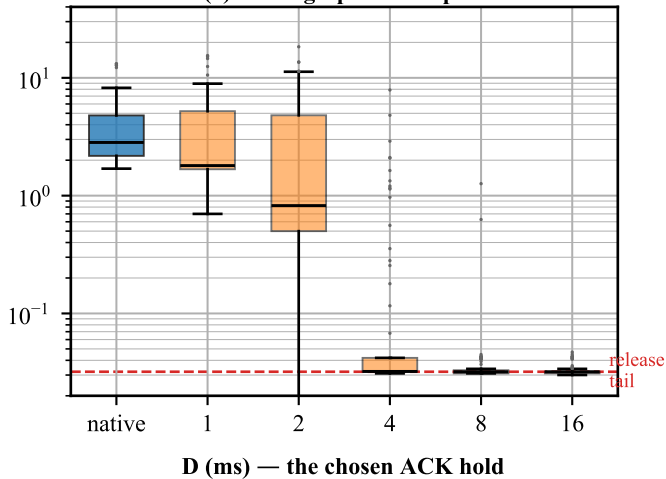
(a) the fingerprint collapses
