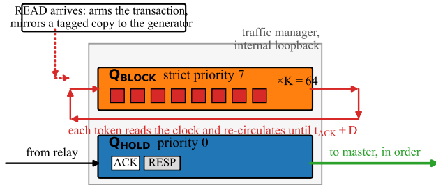
(a) delaying a packet in a chip with no timers
