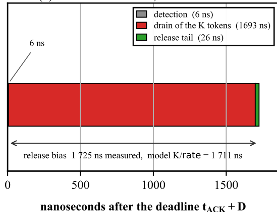
(b) the hold is D + \text{this} ; D = 1\,999\,691\text{ ns}
