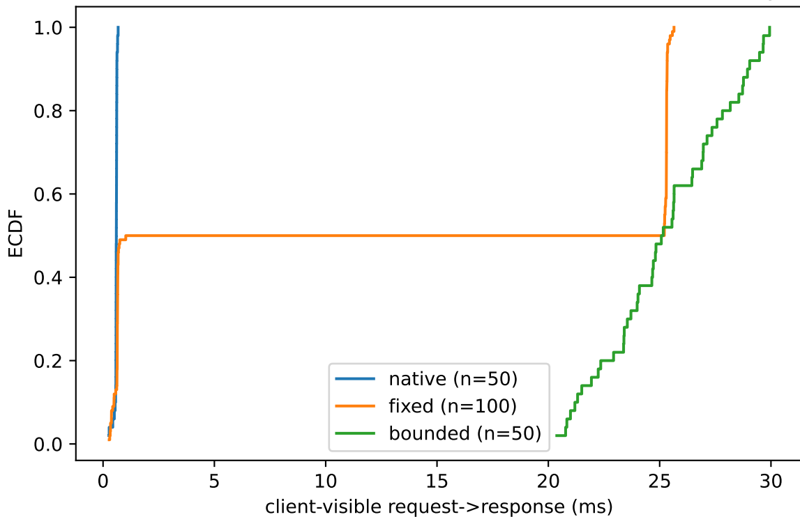
Phase 02: client-visible time ECDF (2407 B READ, full delivery)
