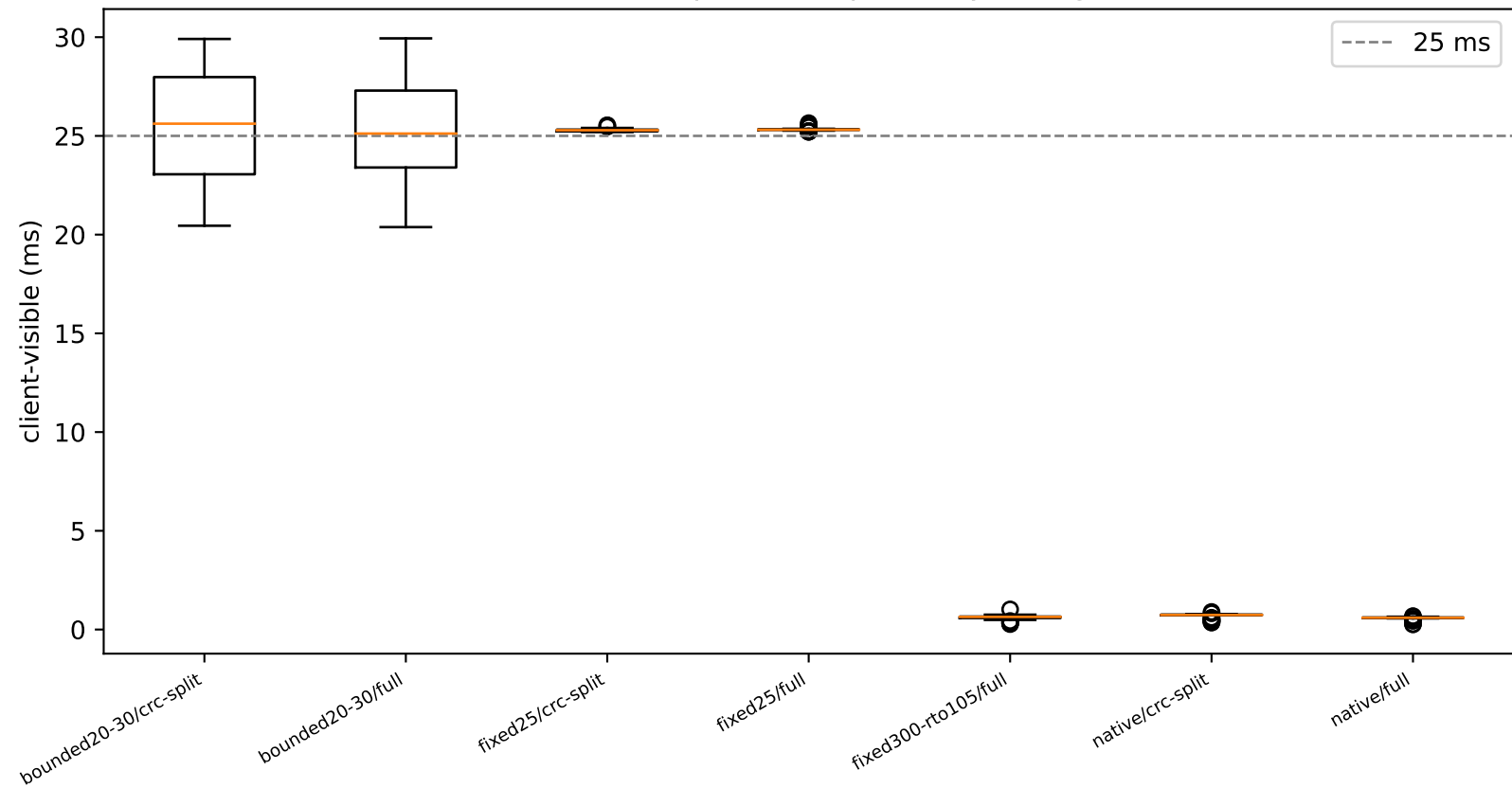
Phase 02: client-visible request->response by config (2407 B READ)
