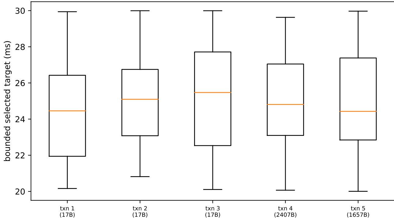
Phase 02 bounded: target by transaction position (no position->target mapping after fix)
