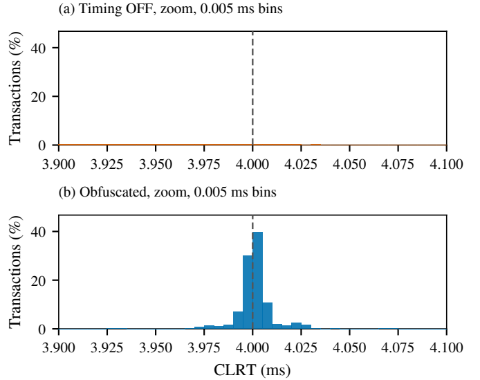
Fig. 6. The released interval, resolved. The same measurements as Figure 5 on 0.005 ms bins within 0.10 ms of the configured CLRT_{new} (dashed). The ordinate is still the percentage of that arm's entire sample, not of the window, so the bars are directly comparable with the other figures. The window holds 13.58% of (a) and 99.86% of (b).
