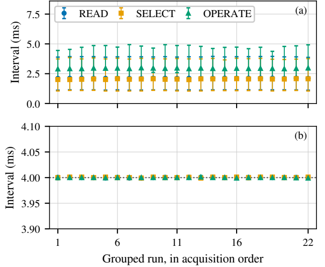
Fig. 8. Per-run medians and interquartile ranges, in acquisition order. Panel (b) uses a magnified ordinate spanning 0.20 ms. The runs are one campaign, not independent replications.
