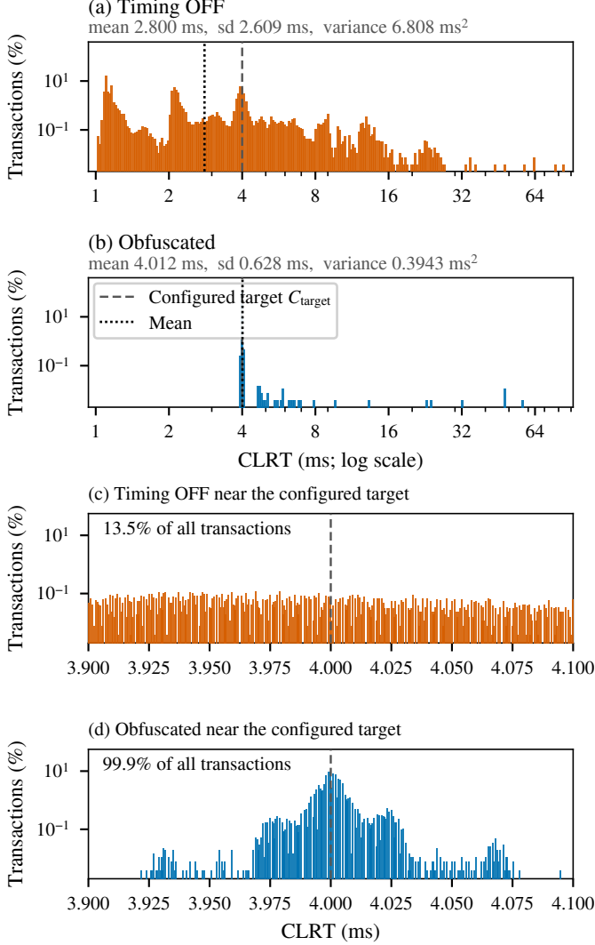
Fig. 6. Measured READ CLRT before and after obfuscation. (a) and (b) show the full measured range on logarithmic axes, on common bins and identical limits. (c) and (d) show a linear window of 0.10 ms either side of the configured target. Bars are the percentage of that arm’s own transactions in each bin, and in (c) and (d) the denominator is still the arm’s full sample, so the share falling inside the window is a share of everything measured. The dashed line is the configured target, a policy value; the dotted line is the measured mean. Nothing is smoothed and no tail is clipped.
