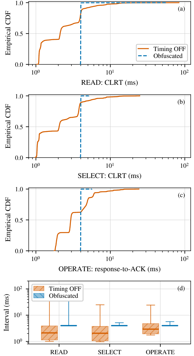
Fig. 5. Measured interval per transaction class, over 22 grouped runs. (a) READ and (b) the SELECT phase of SBO report the cross-layer response time; (c) OPERATE reports the master-visible response-to-ACK interval, which is a different anchor and not a complete SBO transaction. The abscissa is logarithmic and spans the full support, so no observation is clipped. (d) The same measurements as quartiles, with whiskers spanning the full support.
