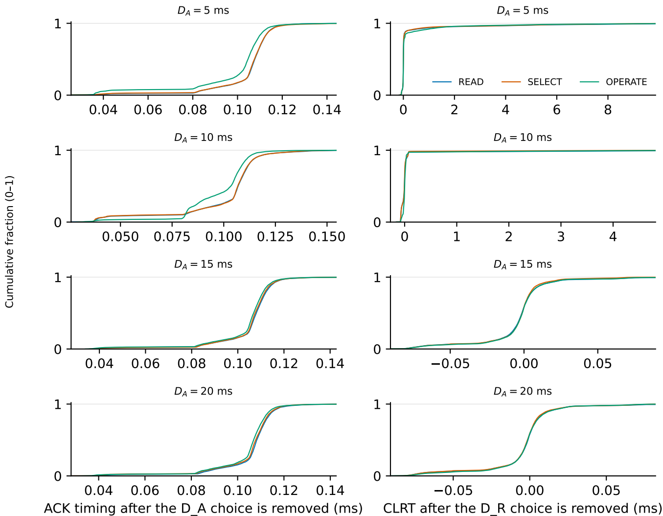
Held-out packet-timing distributions by operation (after subtracting the nearest configured D_A/D_R choice)
