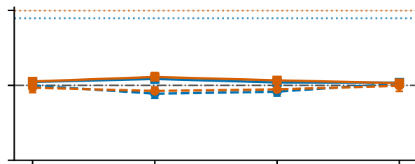
READ vs SBO · 200-bin CLRT histogram
