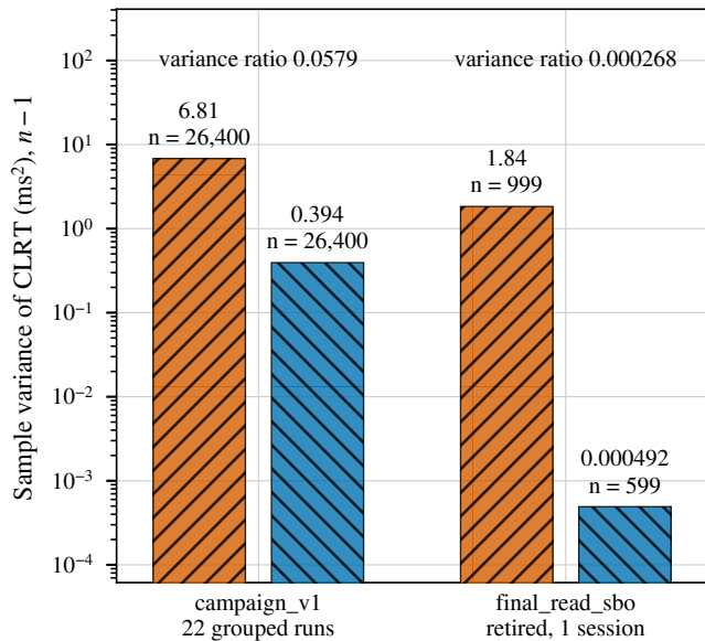
(b) sample variance, per corpus and arm
