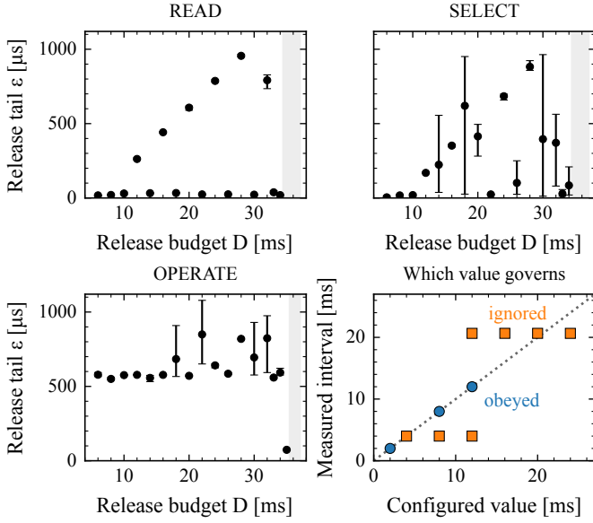
Fig. 7. The release tail \varepsilon against the budget D for each class, over three installs of each setting; whiskers span them, and in the shaded region the reservoir spends its pass budget and releases early. OPERATE is timed from the request, so its \varepsilon is the acknowledgment’s arrival beyond T_0 + D_A . Lower right, each configured quantity that could set a master-visible OPERATE interval, against the interval it would set: the configured CLRT new is obeyed, and the control plane’s offsets A and R - A are ignored.
