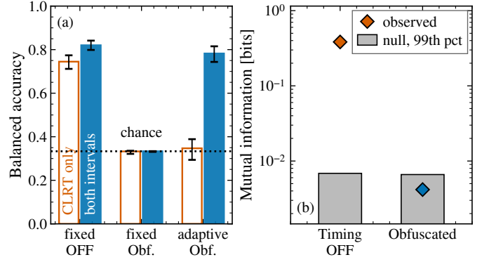
Fig. 8. Transaction-class leakage under the two attacker models, leaving out one grouped run at a time. (a) Balanced accuracy by attacker condition and feature set. The abscissa names the training condition and the arm it is tested on: fixed on Timing OFF, the same fixed model on Obfuscated traffic, and a model retrained on Obfuscated traffic. Whiskers span the 22 held-out runs and are not a confidence interval. (b) Mutual information between the CLRT and the class, against a within-run permutation null.
