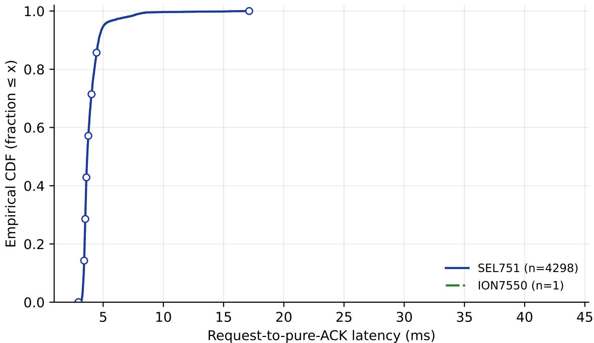
Request-to-pure-ACK latency CDF (separate-ACK devices) (n=4299; SEL751=4298, ION7550=1)
