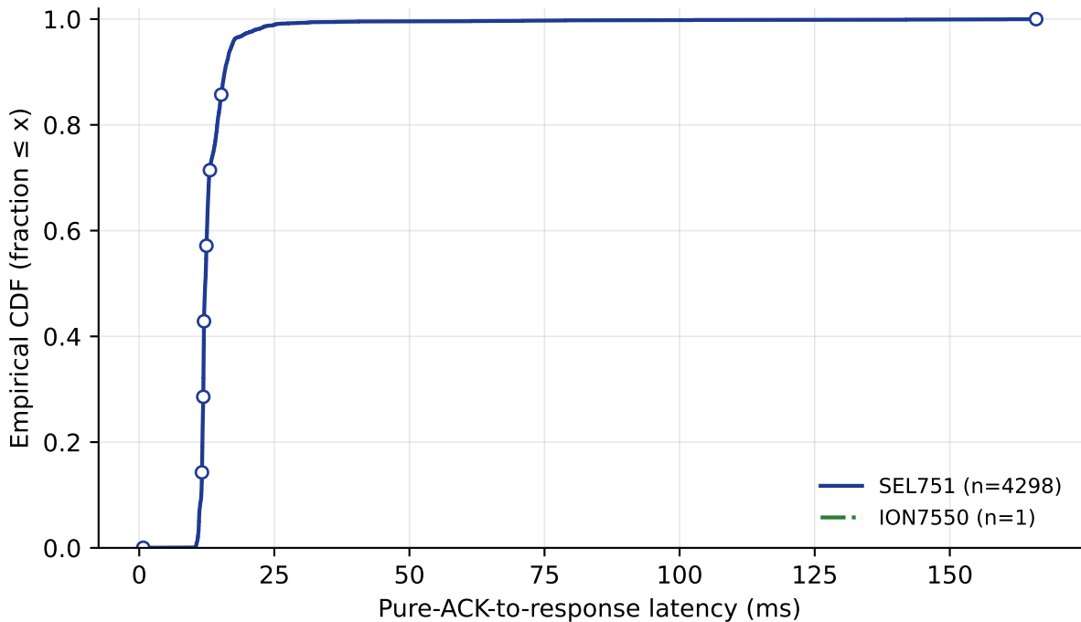
Pure-ACK-to-response latency CDF (separate-ACK devices) (n=4299; SEL751=4298, ION7550=1)
