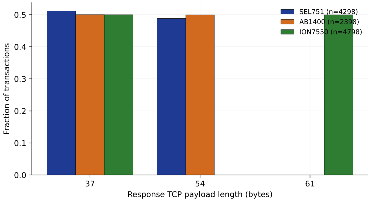
Response-size distribution by device (n=11494)
