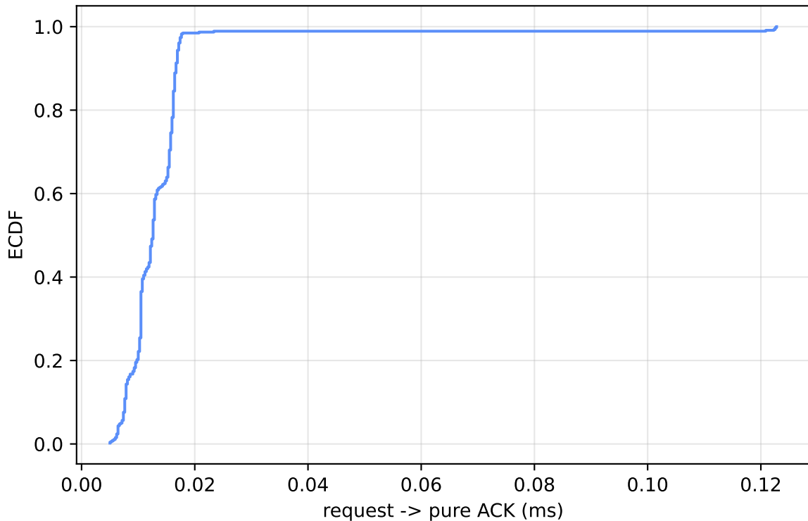
Phase 03A: request->pure-ACK CDF (separated non-first) pure ACK is emitted promptly ( \sim 0.01 ms), not at the response delay
