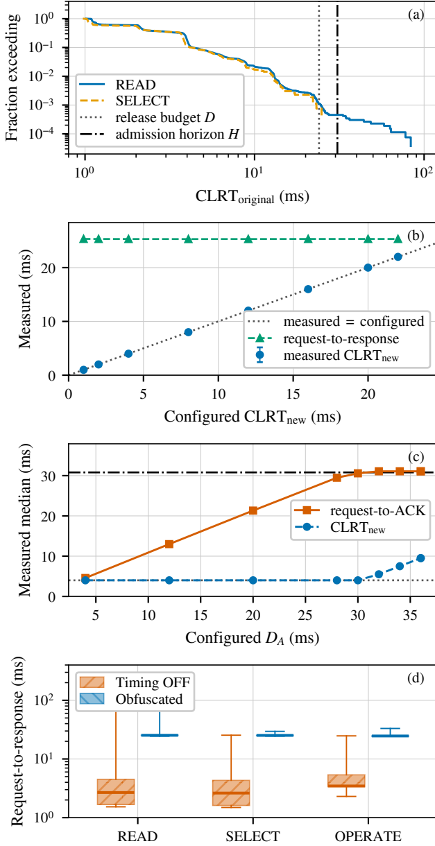
Fig. 10. The release policy is programmable and bounded on both sides. (a) Timing OFF read-lane tail against the budget D and the horizon H . (b) At D = 24 ms the measured CLRT new follows the configured CLRT new while the response latency stays fixed. (c) Raising D_A saturates near H . (d) End-to-end response time per class.
