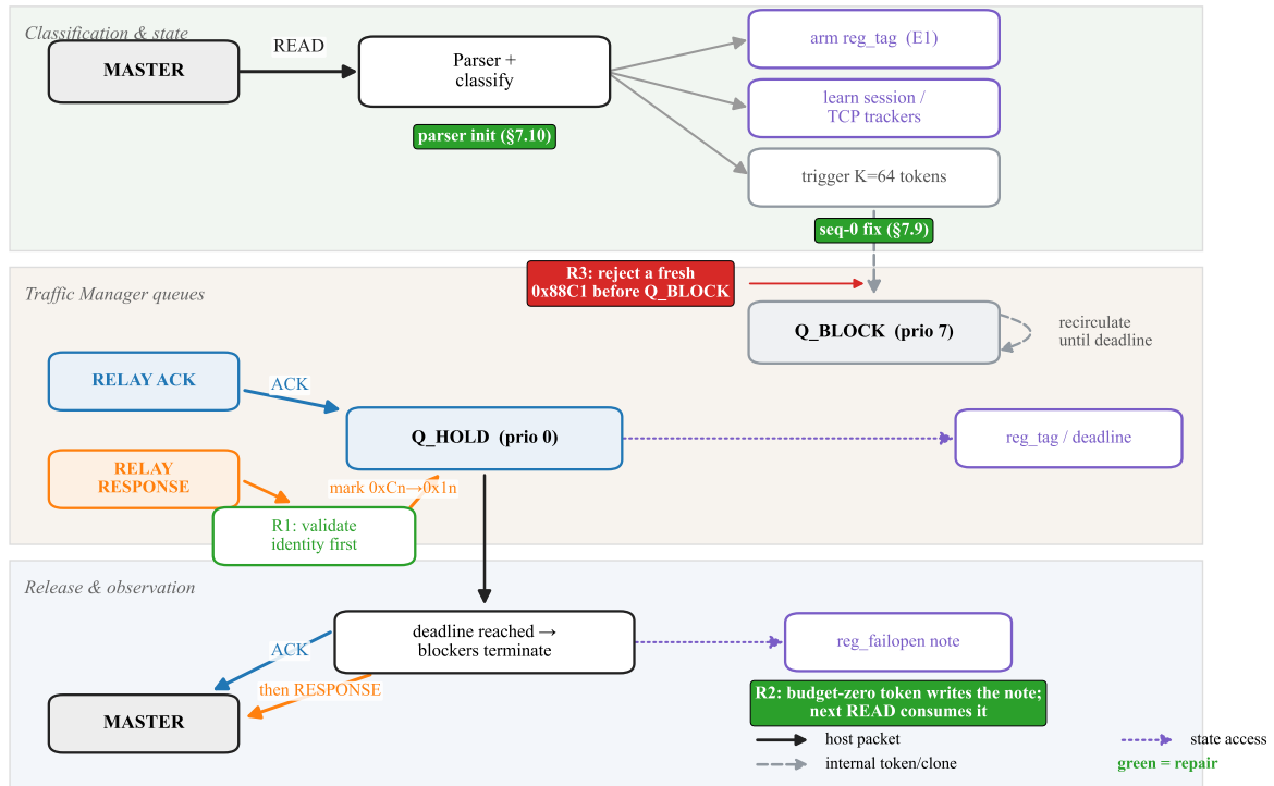
Figure 8: The end-to-end Defense 3 lifecycle, with the repairs on the paths they guard. A READ arms the state (reg_tag, E1), learns the session, and triggers K=64 tokens into Q_BLOCK (strict priority 7), which recirculate until the deadline. The relay’s ACK and an in-window RESPONSE share Q_HOLD (priority 0), so the ACK leaves first; at the deadline the blockers terminate and the ACK, then the RESPONSE, reach the master. Repairs (green/red): R1 validates a RESPONSE’s identity before it marks the state; R2 a budget-zero token writes a reg_failopen note that the next READ consumes; R3 rejects a fresh non-generator 0x88C1 before Q_BLOCK; the parser-init (§8.10) and sequence-zero (§8.9) fixes are small callouts. Solid = host packets, dashed = internal tokens, dotted = state accesses.
