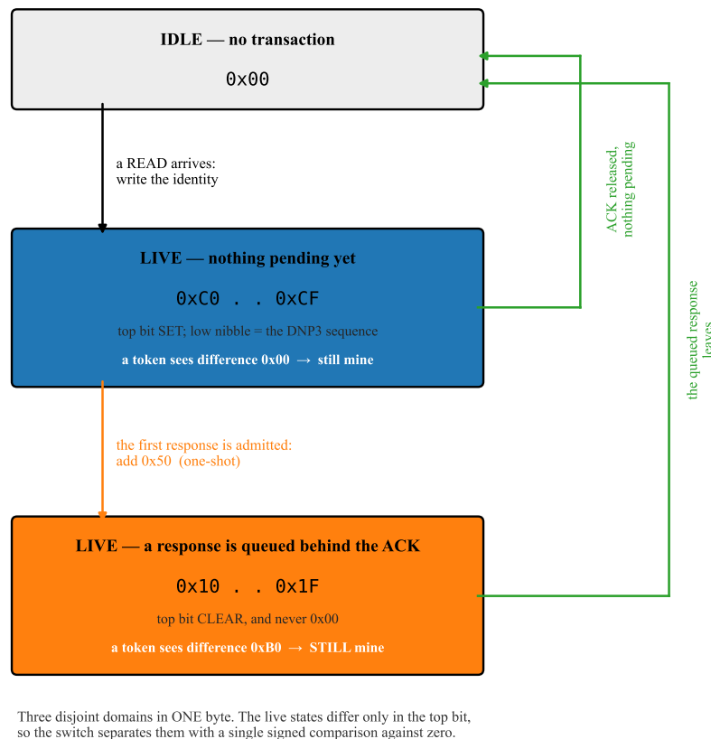
Figure 8: The transaction state machine: three disjoint domains inside one byte. The two live states differ only in the top bit, so the switch separates them with a single signed comparison against zero (§7). The white lines inside the live boxes are what a circulating blocker token computes — the identity it carries minus the value it finds. Because the marking transition adds a constant rather than overwriting, that difference is 0x00 before marking and 0xB0 after, so one extra table entry covers all sixteen identities and the reservoir survives the state change. Source: figures/src/fig5_statemachine.py .
