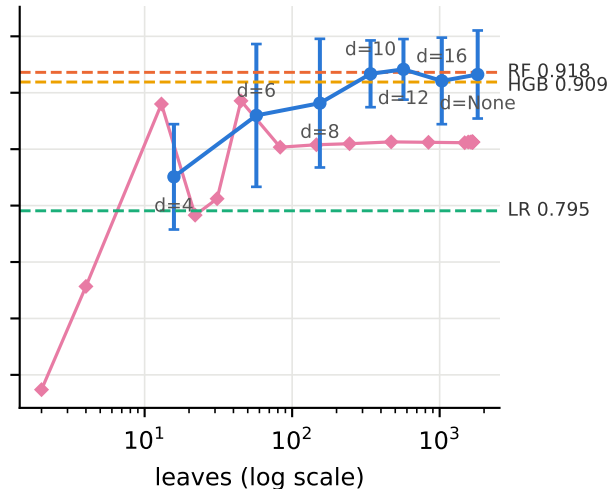
full (Zeek) (Bayes acc. ceiling 0.970)
