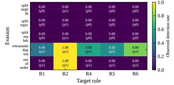
Figure 12: TCP-segmentation evasion (E23): observed per-cell drop rate over 10 trials/cell (250 trials), each cell reset-isolated; cell text is observed rate (predicted in parens). Header-split evasions defeat every rule including the source-keyed R2; only retransmit-dup (intact PUBLISH on the wire) yields parse-dependent detection, and only probabilistically. The R5 column does not exercise genuine fanout (single-PUBLISH base attack) and is shown for completeness.
