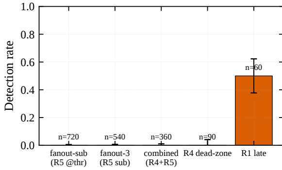
Figure 11: Per-strategy adaptive-mimicry detection rate (E21) over 30 campaigns; error bars are Wilson 95% CIs. Only r1-late produces any detection (R1 on the second replay, 0.50); every sub-threshold strategy evades entirely (0/N with Wilson upper bounds < 5%). Cross-strategy BCa F_1 = 0.033 [0.022, 0.049].
