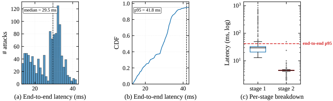
Figure 14: End-to-end detection latency on 1200 attack events from the stochastic experiment: (a) histogram, (b) empirical CDF, (c) per-stage box plot on log scale. Stage 1 = send → digest arrival (generator + Tofino 1 pipeline + gRPC transport); stage 2 = digest arrival → controller decision (Python arbitration); end-to-end = stage 1 + stage 2. Medians 29.5/4.5/34.0 ms; p95 values 41.8/4.8/46.6 ms. Latency is restricted to attack events because the benign workload interposes inter-trial state-reset barriers ( \sim 2.7 s) between trials; those barriers are driver-side synchronization, not per-event detection latency, so pooling them would overstate the on-path tail.
