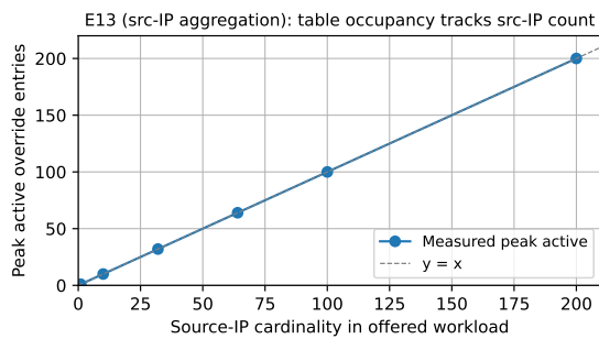
Figure 9: Override-table occupancy under source-IP aggregation (E13). Peak active override-table entries versus offered source-IP cardinality at 500 pps per window, averaged over a 5 s TTL. Measurements fall exactly on y = x : one table entry per distinct source IP, independent of 5-tuple fanout. Zero installs are rejected up to 200 source IPs in our deployment pipeline.
