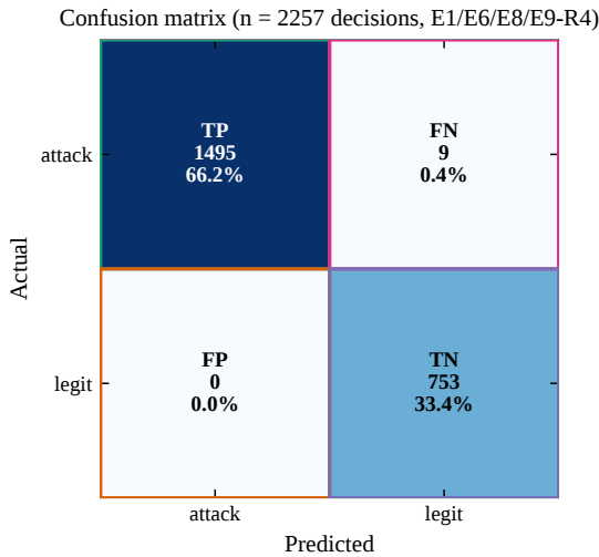
Figure 4: Pooled confusion matrix across the four scoring experiments (E1 attack detection, E6 oversize, E8 stochastic, E9 R4 evasion; n = 2257 decisions). Zero false positives and nine false negatives; the nine FNs come from the stochastic trials of E8 and match its recall of 0.992. E4 is an arbiter ablation (RAT disabled), not a detector-scoring run, so it is excluded from the pooled detector matrix.
