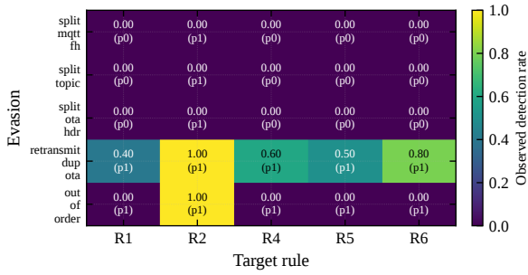
Figure 11: TCP-segmentation evasion (E23): observed per-cell drop rate over 10 trials/cell (250 trials), each cell reset-isolated; cell text is observed rate (predicted in parens). Header-split evasions defeat every rule including the source-keyed R2; only retransmit-dup (intact PUBLISH on the wire) yields parse-dependent detection, and only probabilistically. The R5 column does not exercise genuine fanout (single-PUBLISH base attack) and is shown for completeness.
