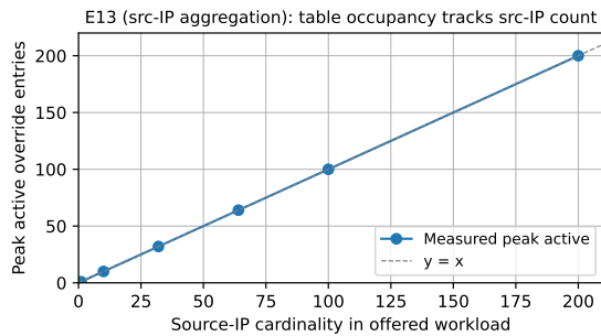
Figure 9: Override-table occupancy under source-IP aggregation (E13). Peak active override-table entries versus offered source-IP cardinality at 500 pps per window, averaged over a 5 s TTL. Measurements fall exactly on y = x : one table entry per distinct source IP, independent of 5-tuple fanout. Zero installs are rejected up to 200 source IPs in our deployment pipeline.
