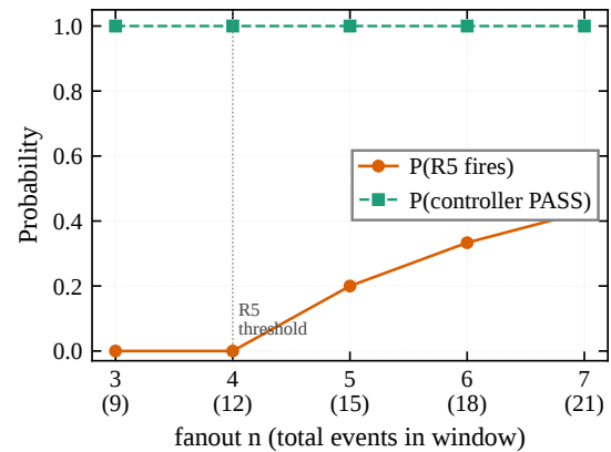
Figure 10: R5 sensitivity as a function of fanout size: P(R5 \text{ fires}) grows linearly above threshold 4, characterizing the rule's intrinsic counter. On the deployed build R5's counter is r2-gated, so an authorized fanout never fires R5 (§6.4); the authorized-rollout PASS rate is 1.0 trivially, with no R5 fire to demote.
