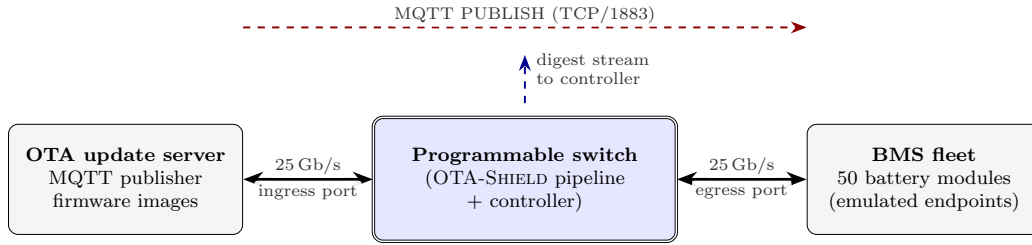
Figure 12: Testbed topology. An OTA update server and a 50-unit BMS fleet connect to a programmable switch through data-plane links configured at 25 Gb/s with RS-FEC (link capability; the experiments in this paper do not offer traffic at that rate). A separate management LAN carries control-plane gRPC traffic.
