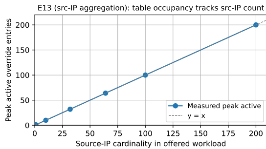
Figure D.2: Override-table occupancy under source-IP aggregation (E13). Peak active override-table entries versus offered source-IP cardinality at 500 pps per window, averaged over a 5 s TTL. Measurements fall exactly on y = x : one table entry per distinct source IP, independent of 5-tuple fanout. Zero installs are rejected up to 200 source IPs in our deployment pipeline.
