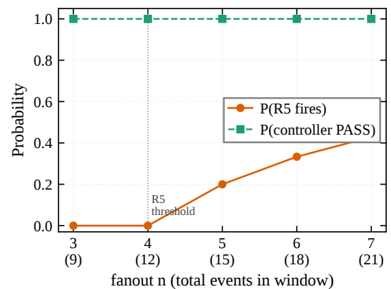
Figure D.3: R5 sensitivity as a function of fanout size: P(R5 \text{ fires}) grows linearly above threshold 4, characterizing the rule's intrinsic counter. On the deployed build R5's counter is r2-gated, so an authorized fanout never fires R5 (§6.4); the authorized-rollout PASS rate is 1.0 trivially, with no R5 fire to demote.
