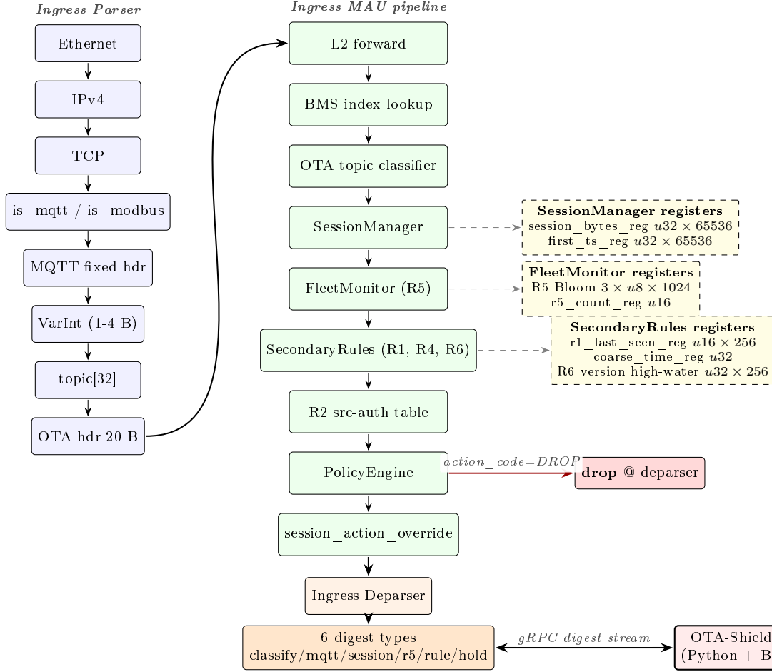
Figure 4: P4 ingress pipeline. Dashed arrows connect MAU control blocks to their stateful registers. Topic and OTA header use fixed-size slots; other parameter combinations are discussed in §6.7.
