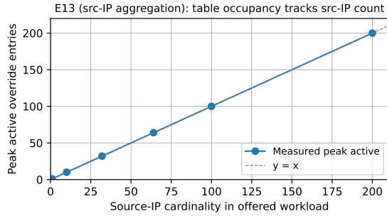
Figure 15: Override-table occupancy under source-IP aggregation (E13). Peak active override-table entries versus offered source-IP cardinality at 500 pps per window, averaged over a 5 s TTL. Measurements fall exactly on y = x : one table entry per distinct source IP, independent of 5-tuple fanout. Zero installs are rejected up to 200 source IPs in our deployment pipeline.
