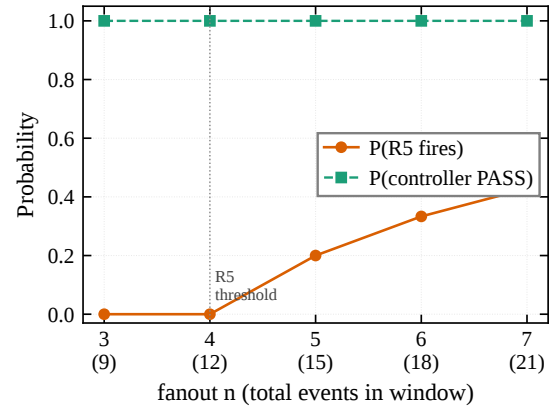
Figure 10: R5 sensitivity as a function of fanout size: P(R5 \text{ fires}) grows linearly above threshold 4, characterizing the rule's intrinsic counter. On the deployed build R5's counter is r2 -gated, so an authorized fanout never fires R5 (§6.4); the authorized-rollout PASS rate is 1.0 trivially, with no R5 fire to demote.
