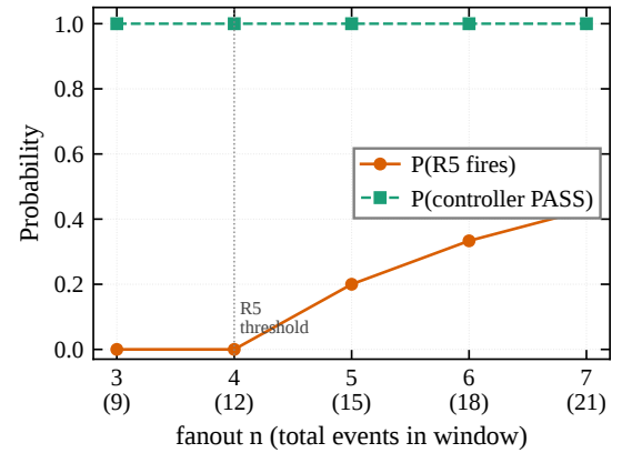
Figure F.3: R5 sensitivity as a function of fanout size: P(R5 \text{ fires}) grows linearly above threshold 4, characterizing the rule's intrinsic counter. On the deployed build R5's counter is r2-gated, so an authorized fanout never fires R5 (§6.4); the authorized-rollout PASS rate is 1.0 trivially, with no R5 fire to demote.
