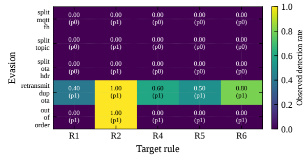
Figure F.4: TCP-segmentation evasion (E23): observed per-cell drop rate over 10 trials/cell (250 trials), each cell reset-isolated; cell text is observed rate (predicted in parens). Header-split evasions defeat every rule including the source-keyed R2; only retransmit-dup (intact PUBLISH on the wire) yields parse-dependent detection, and only probabilistically. The R5 column does not exercise genuine fanout (single-PUBLISH base attack) and is shown for completeness.
