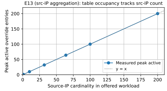
Figure F.2: Override-table occupancy under source-IP aggregation (E13). Peak active override-table entries versus offered source-IP cardinality at 500 pps per window, averaged over a 5 s TTL. Measurements fall exactly on y = x : one table entry per distinct source IP, independent of 5-tuple fanout. Zero installs are rejected up to 200 source IPs in our deployment pipeline.
