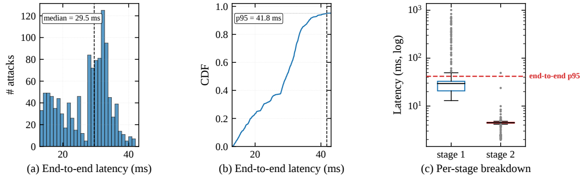
Figure D.2: End-to-end detection latency on 1200 attack events from the stochastic experiment: (a) histogram, (b) empirical CDF, (c) per-stage box plot on log scale. Stage 1 = send \rightarrow digest arrival (generator + Tofino 1 pipeline + gRPC transport); stage 2 = digest arrival \rightarrow controller decision (Python arbitration); end-to-end = stage 1 + stage 2. Medians 29.5/4.5/34.0 ms; p95 values 41.8/4.8/46.6 ms. Latency is restricted to attack events because the benign workload interposes inter-trial state-reset barriers ( \sim 2.7 s) between trials; those barriers are driver-side synchronization, not per-event detection latency, so pooling them would overstate the on-path tail.
