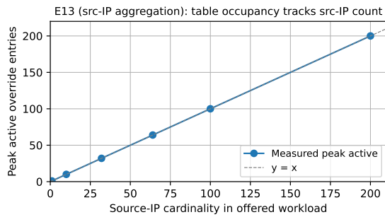
Figure D.3: Override-table occupancy under source-IP aggregation (E13). Peak active override-table entries versus offered source-IP cardinality at 500 pps per window, averaged over a 5 s TTL. Measurements fall exactly on y = x : one table entry per distinct source IP, independent of 5-tuple fanout. Zero installs are rejected up to 200 source IPs in our deployment pipeline.
