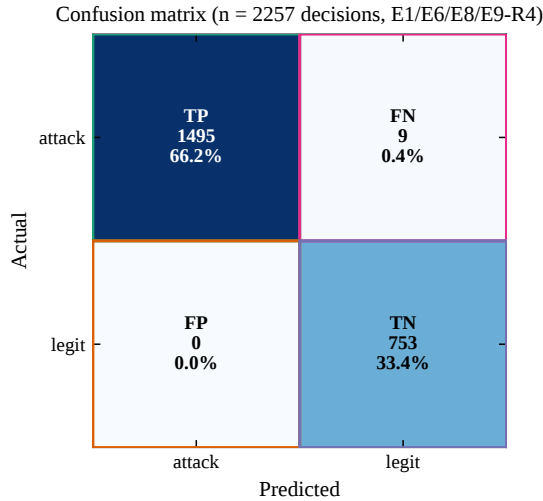
Figure 5: Where the detector’s errors fall: pooled confusion matrix over E1, E6, E8, and E9 ( n = 2257 decisions). Zero false positives and nine false negatives; the nine FNs come from the stochastic trials of E8 and match its recall of 0.992. E4 is an arbiter ablation (RAT disabled), not a detector-scoring run, so it is excluded from the pooled detector matrix.
