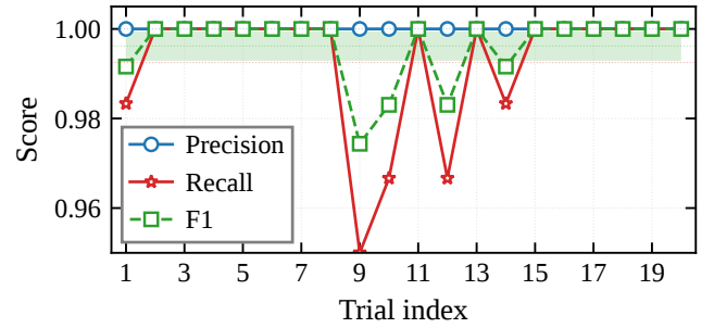
Figure 7: Per-trial precision, recall, and F_1 across the 20 stochastic E8 trials, with the F_1 bootstrap 95% CI band shaded. The narrow dispersion shows that stochastic performance stays close to the CI interval reported for E8 in Table 7.
