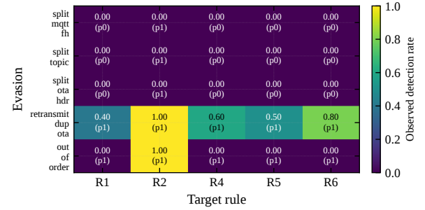
Figure 12: E23 TCP-segmentation evasion battery: observed per-cell drop rate over 10 trials/cell (250 trials), each cell reset-isolated; cell text is observed rate (predicted in parens). Header-split evasions defeat every rule including the source-keyed R2; only retransmit-dup (intact PUBLISH on the wire) yields parse-dependent detection, and only probabilistically. The R5 column does not exercise genuine fanout (single-PUBLISH base attack) and is shown for completeness.
