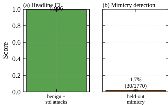
Figure 13: The two headline numbers, shown co-equal on a common [0, 1] scale: (a) naive fleet-fanout detection F_1 = 0.996 (E8) versus (b) adaptive-mimicry coverage 1.7% (E21). The headline applies to the designed naive family; an adversary who reshapes cadence faces the right-hand number.
