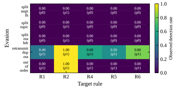
Figure 11: TCP-segmentation evasion (E23): observed per-cell drop rate over 10 trials/cell (250 trials), each cell reset-isolated; cell text is observed rate (predicted in parens). Header-split evasions defeat every rule including the source-keyed R2; only retransmit-dup (intact PUBLISH on the wire) yields parse-dependent detection, and only probabilistically. The R5 column does not exercise genuine fanout (single-PUBLISH base attack) and is shown for completeness.
