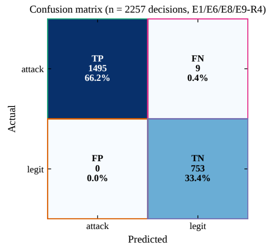
Figure 4: Where the detector’s errors fall: pooled confusion matrix over E1, E6, E8, and E9 ( n = 2257 decisions). Zero false positives and nine false negatives; the nine FNs come from the stochastic trials of E8 and match its recall of 0.992. E4 is an arbiter ablation (RAT disabled), not a detector-scoring run, so it is excluded from the pooled detector matrix.
