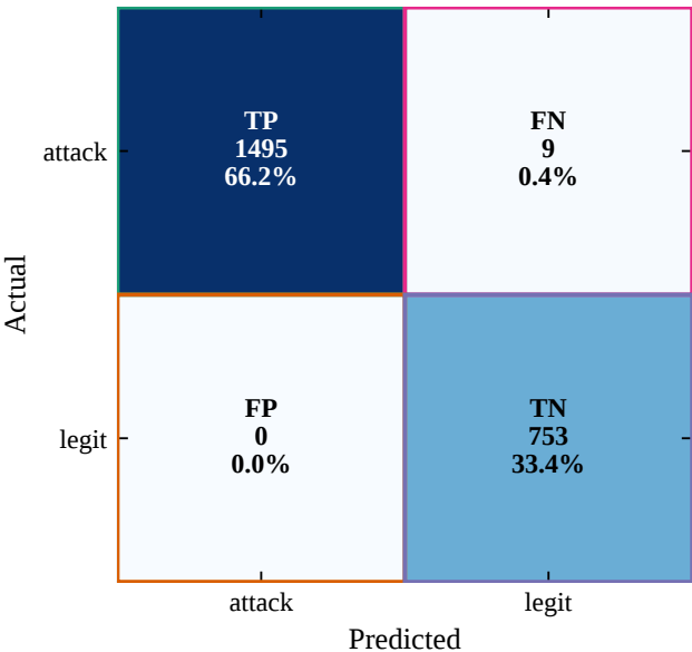
Confusion matrix (n = 2257 decisions, E1/E6/E8/E9-R4)
