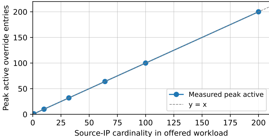
E13 (src-IP aggregation): table occupancy tracks src-IP count
