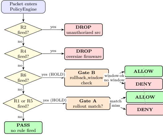
Figure 3: Policy decision flowchart. All rule fires emit a hold_digest to the controller. R2 (unauthorized source) and R4 (oversize payload) remain terminal DROP decisions. R1 (rapid replay) and R6 (version rollback) enter control-plane arbitration: Gate A demotes an R1 fire that matches an active authorized rollout to PASS (R5 cannot reach Gate A on the deployed build, its counter being r2-gated , §6.4), and Gate B demotes an R6 fire to PASS only when the active RAT entry carries an explicit rollback_window covering the observed version. Any other HOLD becomes a DROP override. Override entries expire after 5 s (fail-closed).
