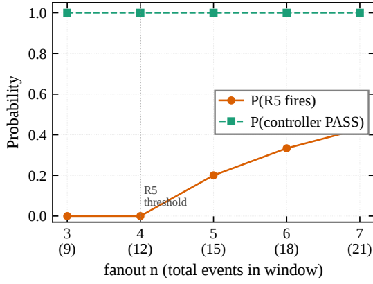
Figure 10: R5 sensitivity as a function of fanout size: P(R5 \text{ fires}) grows linearly above threshold 4, characterizing the rule's intrinsic counter. On the deployed build R5's counter is r2-gated, so an authorized fanout never fires R5 (§6.4); the authorized-rollout PASS rate is 1.0 trivially, with no R5 fire to demote.
