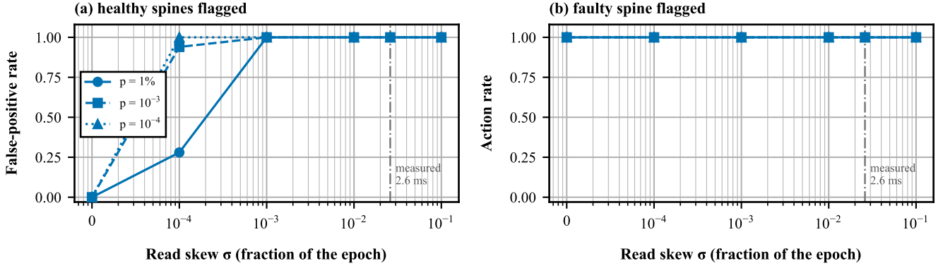
Fig. 4. The zero-byte counter pair against controller read skew, 50 seeds per cell, for three loss rates. (a) Fraction of seeds in which a healthy spine was flagged. (b) Fraction of seeds in which the faulty spine was flagged. At \sigma = 0 the arm is the ledger's information read at one instant and matches the ledger exactly; the vertical line is the best case measured on the switch, a 2.6 ms pairwise read against a 100 ms epoch.
