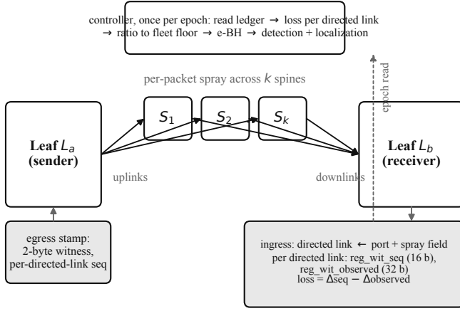
Fig. 1. The receiver ledger on a sprayed leaf-spine fabric. The sending leaf stamps each packet at egress with a two-byte per-directed-link sequence number. The receiving switch reconstructs the directed link from its own ingress port and the spray field, and keeps two registers per directed link: the last sequence number seen and the number of packets seen. Once per epoch the controller reads both registers, takes the difference of their deltas as the loss on that directed link, compares it with the fleet floor, and applies e-BH to name the faulty links.
