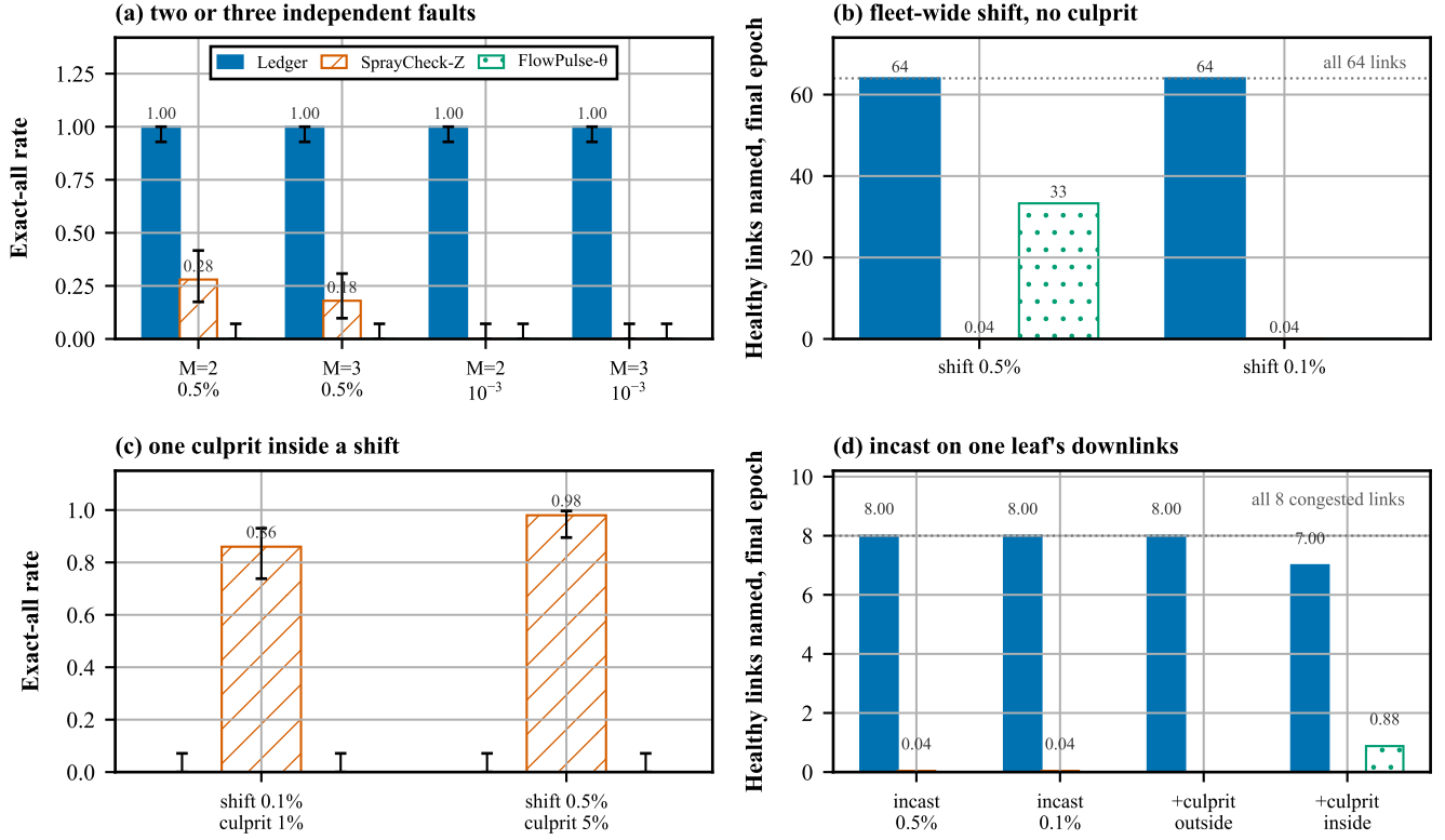
Fig. 7. The correlated-fault gate, 50 seeds per cell over 40 post-onset epochs on 64 directed links. (a) Exact-all rate, with 95 percent intervals, for two and three simultaneous independent faults. (b) Healthy links falsely named at the final epoch under a fleet-wide shift with no culprit, where the correct answer is zero and 64 is every link. (c) Exact-all rate for one culprit embedded in a shift. (d) Healthy links falsely named at the final epoch when the eight downlinks into one leaf carry persistent congestion loss, alone and with a culprit outside or inside the congested set. The ledger holds in (a) and fails in (b), (c), and (d), where SprayCheck-Z holds.
