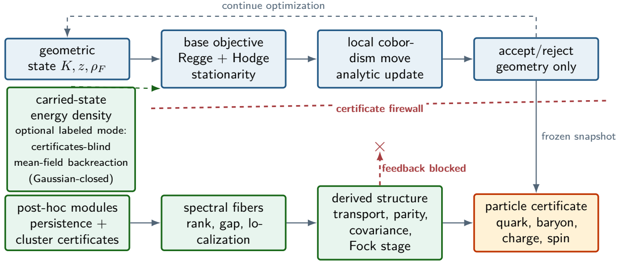
Figure 4: No-feedback emergence protocol. Only the base geometric objective drives optimization. In the certificates-blind backreaction mode the carried state’s energy density may enter that objective; Section 7 records that this remains inside the quasi-free class. Cluster, fiber, color, exchange, and baryon observables are computed from accepted snapshots and cannot feed back into the objective in either emergence mode. Targeted synthesis is a separate, explicitly labeled mode.
