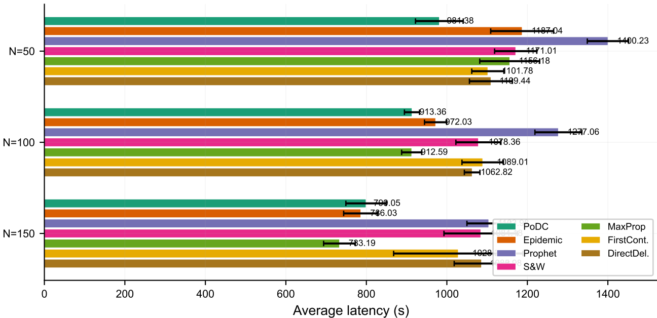
Average latency by protocol and network size
